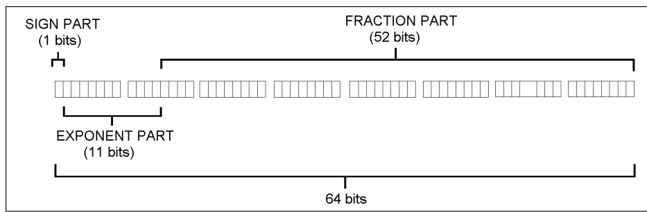
Figure 6-4 64-bit floating-point data
